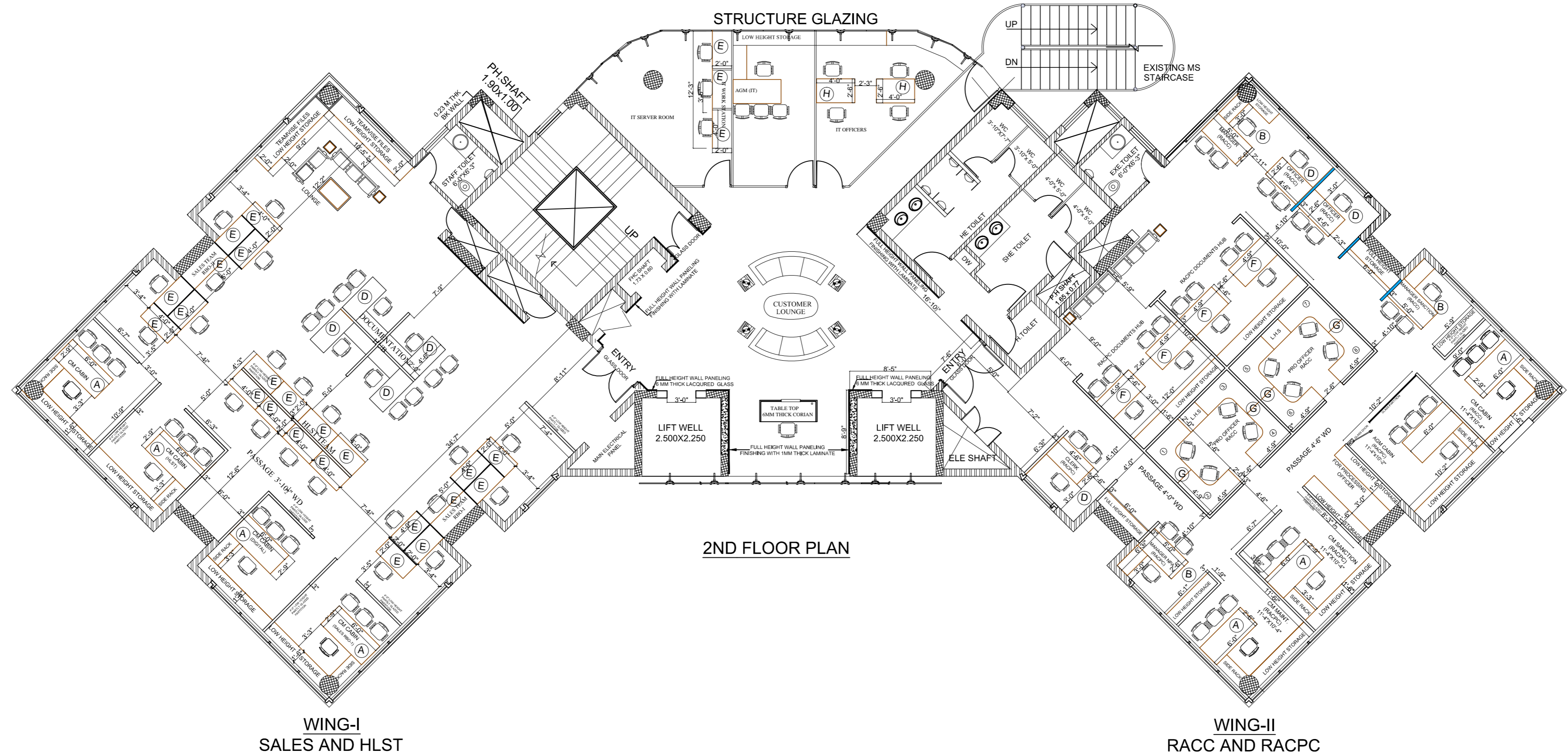
2ND FLOOR PLAN FURNITURE LAYOUT PLAN
